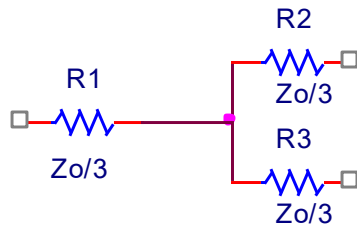
Figure 2: Layout of 2-Way resistive divider
