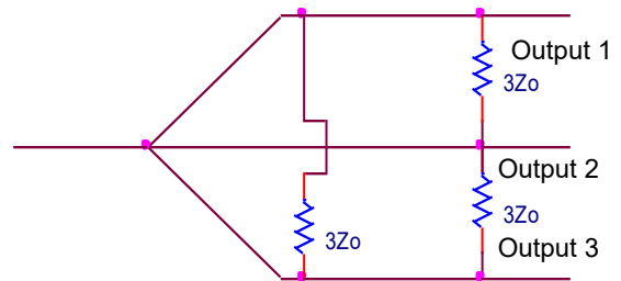
Figure 4: Layout of a 3-Way power divider
