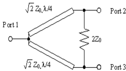
Figure 5: 2-Way Wilkinson power divider
