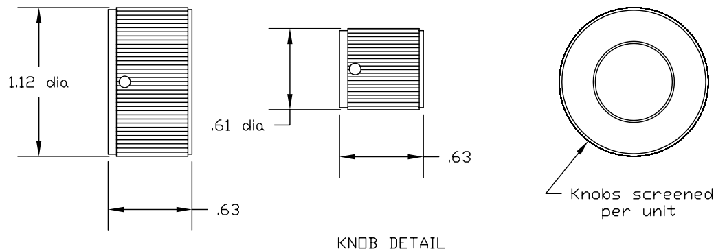
KNOB DETAIL
