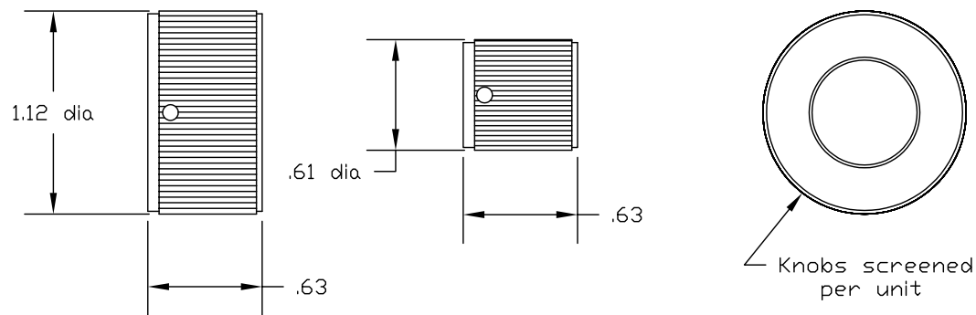
KNOB DETAIL
